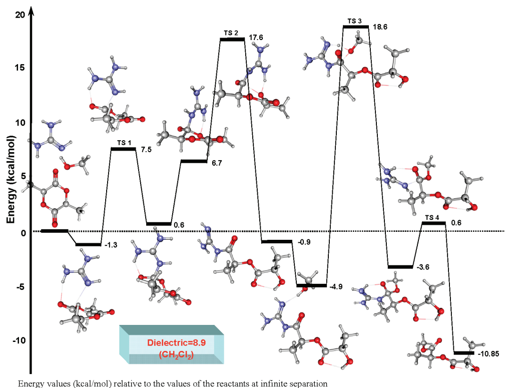
Figure 1. Energy profile for Scheme 1.
