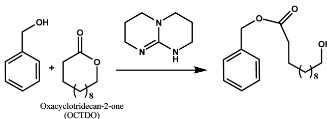
Scheme 4. Ring-Opening Reaction of OCTDO with Benzyl Alcohol (BAol) as Initiator and TBD as Catalyst
